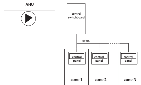
2. Several control panels operating with one AHU
