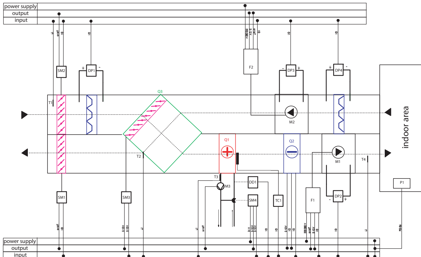
Air handling unit with water heater, plate heat recovery section and evaporator section
