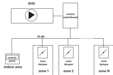
4. Multizone system
