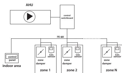
5. Multizone system with CO 2 sensors
